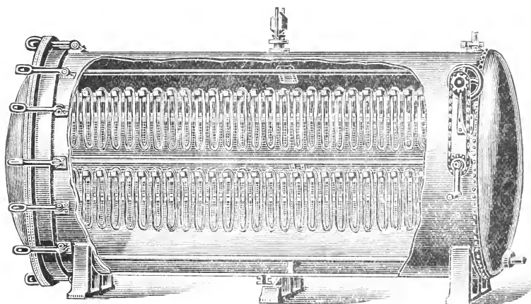
FIG. 37.—Steaming Cottage.
